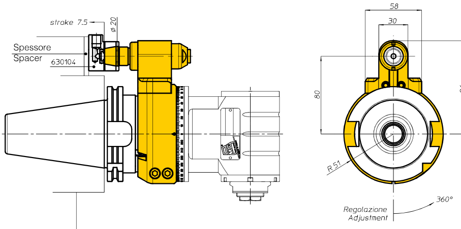
Teste ad angolo TA13.CP, TA16.CP con interasse H=80 Angle heads TA13.CP, TA16.CP with centre distance H=80
