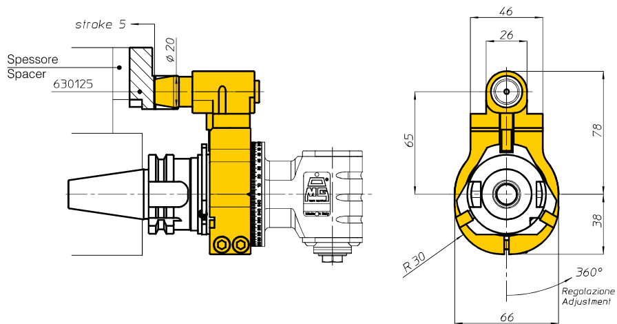
Teste ad angolo TA13.CP, TA16.CP con interasse H=65 Angle heads TA13.CP, TA16.CP with centre distance H=65
