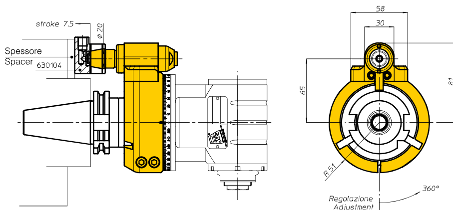
Teste ad angolo TA13.CP, TA16.CP con interasse H=65 Angle heads TA13.CP, TA16.CP with centre distance H=65
