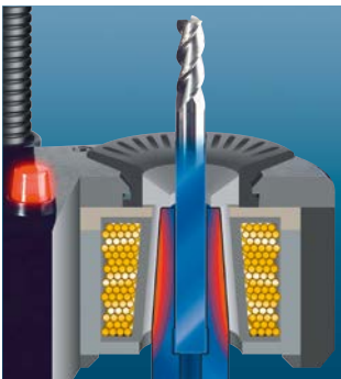
Standard tekercs/Standard coil
