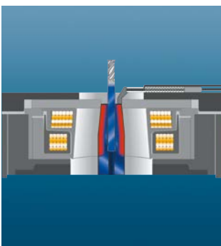
NG-tekercs/NG coil
